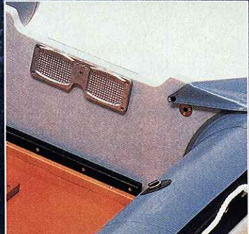
Fiberglass transoms with aluminum pads are found on most Achilles boats.
